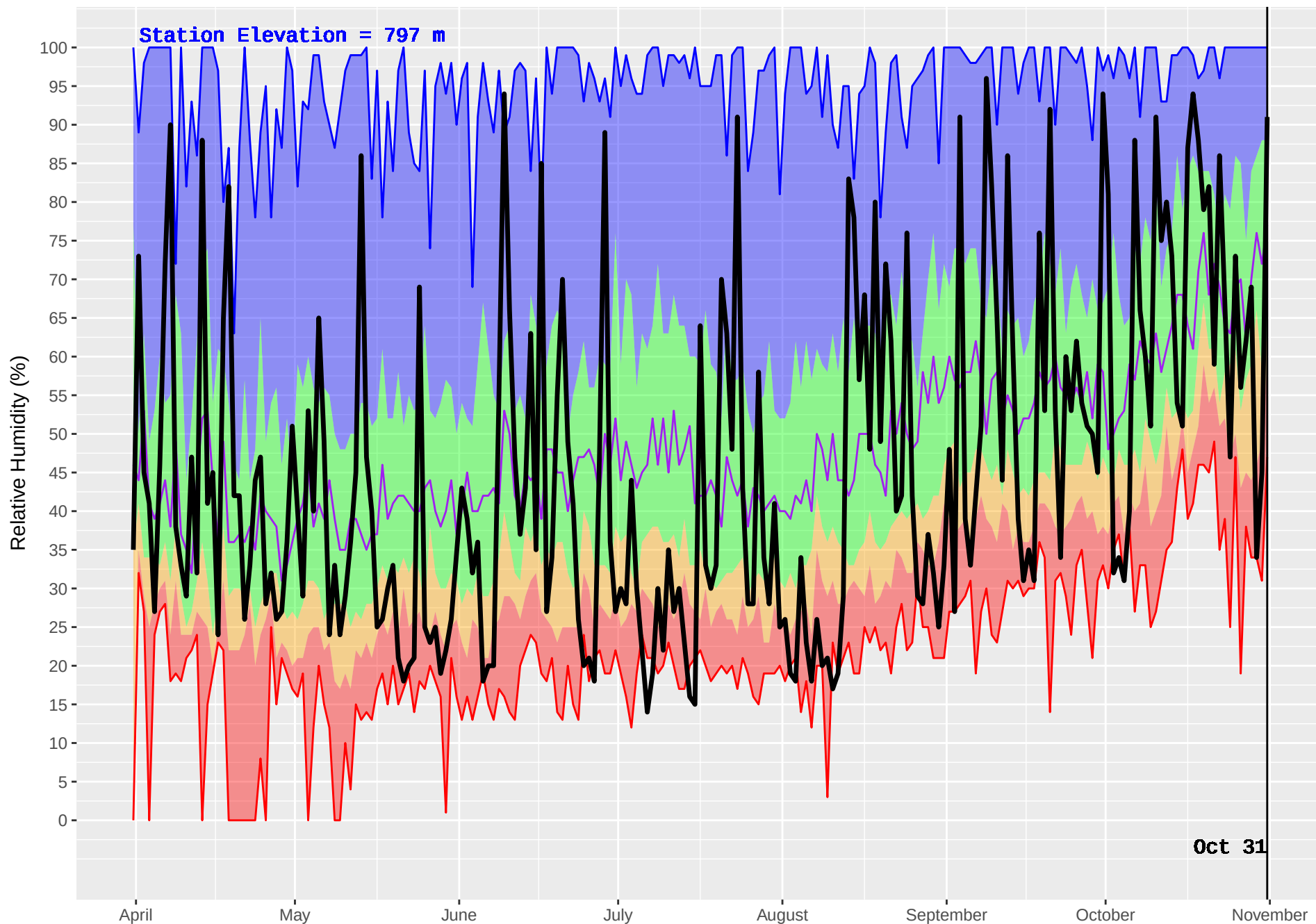
VALEMOUNT HUB (194) : Historical (1970–2016) and Current (2017) Noon Relative Humidity
