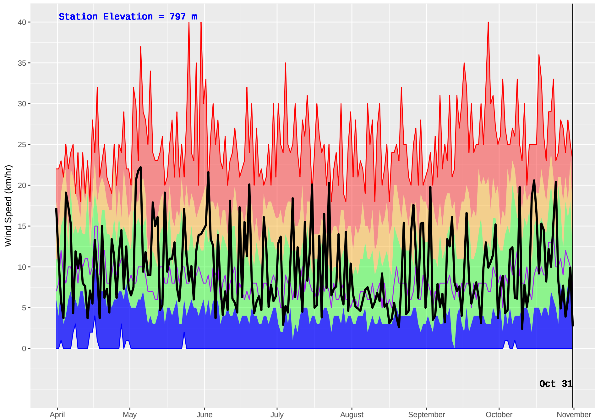
VALEMOUNT HUB (194) : Historical (1970–2016) and Current (2017) Noon Wind Speed
